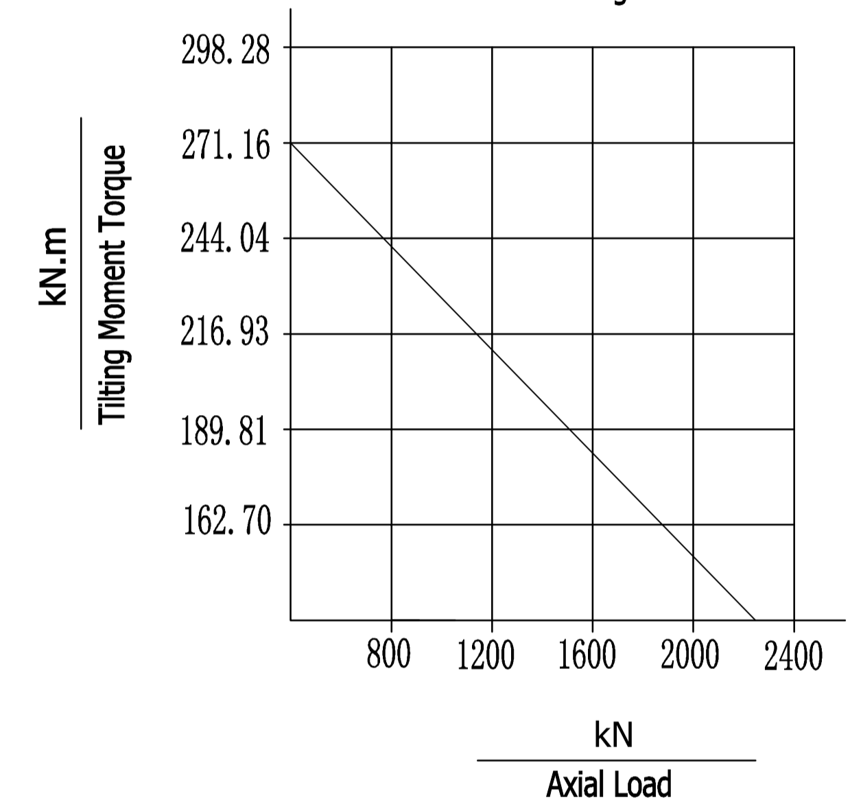
MOMENT LOAD CHART Axial Load & Tilting Moment
